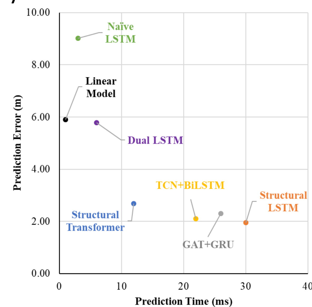
Prediction Speed-Accuracy Trade-off
